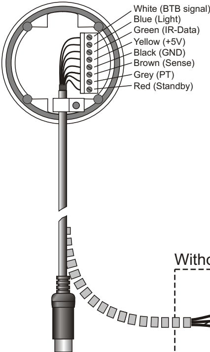
Connection of IR eye to mini DIN connector
